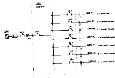
Diagrama Unifilar
